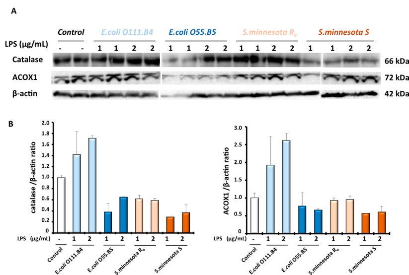
Figure 4. Expression levels of ACOX1 and catalase proteins were evaluated by Western blotting analysis in BV-2 cell extracts after LPS treatment with the four different serotypes (1–2 μg/mL) for 24 h (A). Expression of protein was quantified by densitometry analysis and normalized to the β-actin; (B) and values represent the fold induction relative to the control.
