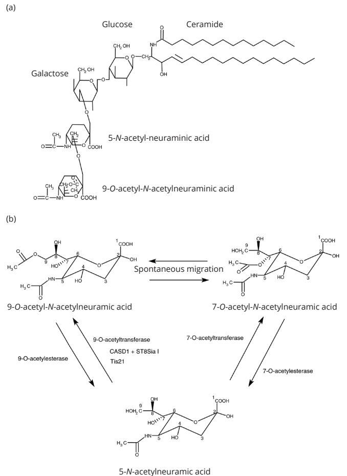
Figure 1 (a) Structure of the disialoganglioside 9- O -acetyl-GD3; (b) chemical and enzymatic relation between the different O -acetylated forms of sialic acid found in gangliosides.
