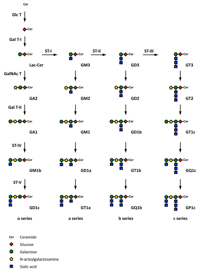
Figure 2 Schematic representation of the main pathway of ganglioside biosynthesis. Cer, ceramide; Lac-Cer, lactosyl ceramide; Glc T, glucosyltransferase; Gal T, galactosyltransferase; GalNAc T, N-acetylgalactosaminyltransferase; ST, sialyltransferase. Diamond, glucose; circle, galactose; pentagon, N-acetylgalactosamine; square, sialic acid.
