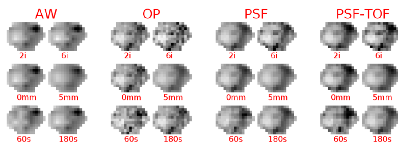
Fig 2. Tumor illustration. Illustration of a tumor (axial slice) reconstructed using different reconstruction settings. Two different images are presented for each reconstruction algorithm studied (AW, OP, PSF and PSF-TOF) corresponding to the minimum and maximum value of the parameters investigated (number of iterations, level of post-filtering and acquisition time). Upper row: variation of the number of iterations (2 and 6 iterations). Middle row: variation of the post-filtering level (0 mm or 5 mm FWHM). Bottom row: variation of the acquisition time for a surrogate of noise in the input data (60 s or 180 s). The grey scale level is identical for each image.
