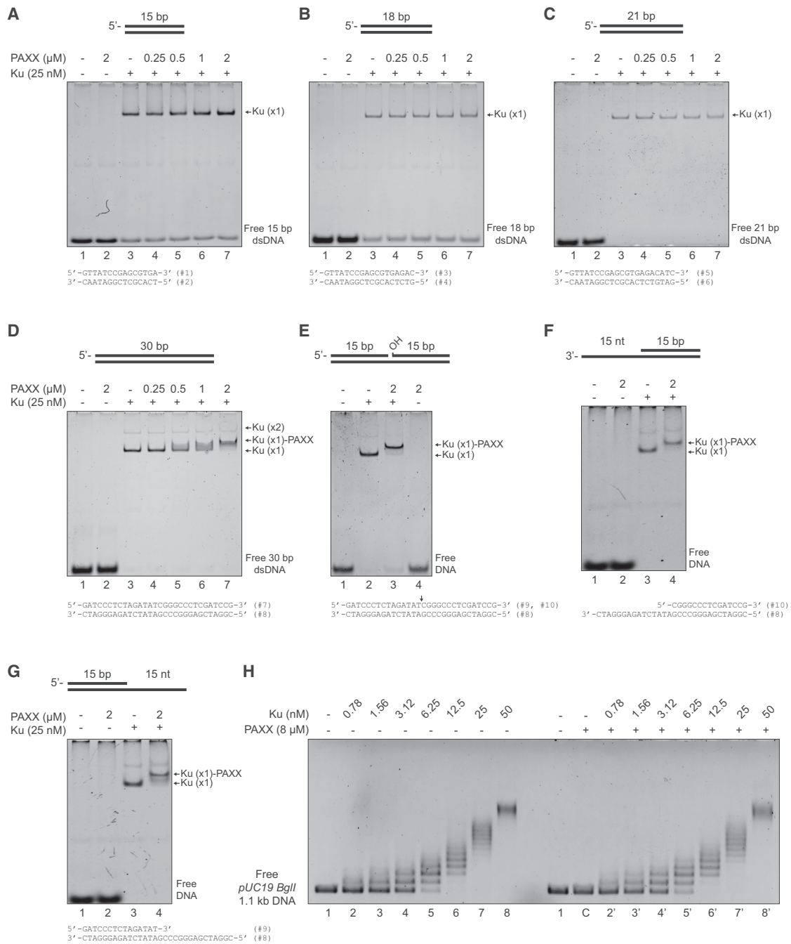
Figure 2. Stable PAXX-Ku-DNA Ternary Complex Requires a Stretch of Bare DNA
