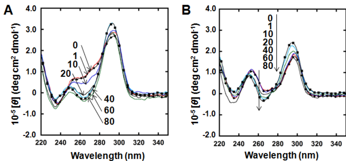
Figure 5. (A) CD spectra of 10 \mu M 22AG with various concentrations of ThT in KCl buffer. (B) CD spectra of 10 \mu M 22AG with various concentrations of ThT in NH 4 OAc buffer. ThT concentrations are 0 \mu M (black with circles), 1 \mu M (red), 10 \mu M (blue), 20 \mu M (purple), 40 \mu M (light blue), 60 \mu M (green), and 80 \mu M (black with squares).
