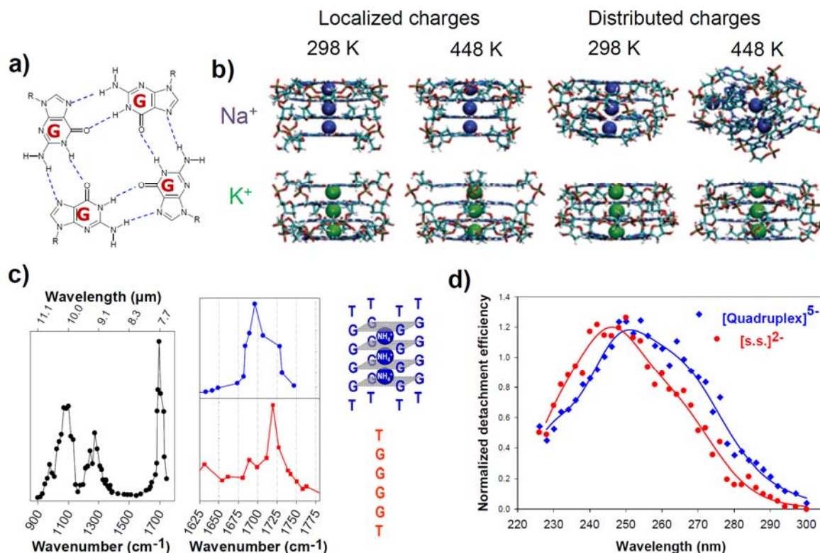
Figure 9: (a) Hydrogen bonding motif of a guanine quartet (G-quartet). (b) Final structures of 500-ns molecular dynamics in the gas phase for parallel-stranded (dGGGG)_4^{5-} , with trapped sodium or potassium. All trajectories are stable except with sodium at high temperature with the distributed charge model. Adapted with permission from Rueda et al., J. Am. Chem. Soc. , 2006, 128, 3608-3619. Copyright 2006 American Chemical Society. (c) Comparative IRMPD ion spectroscopy of single stranded 2- (sequence shown in red) and G-quadruplex 5- (structure shown in blue with the intercalation of 3 ammonium anions between the G quartets) forms of dTGGGGT. Left: full IRMPD spectrum of the G-quadruplex in the gas phase. Right: the carbonyl band shifts to the red upon G-quadruplex formation, due to hydrogen bonding. Adapted with permission from Gabelica et al., J. Am. Chem. Soc. , 2008, 130, 1810-1811. Copyright 2008 American Chemical Society. (d) Comparative UV action spectra of the same single strand and G-quadruplex. UV absorption shifts to the red in the G-quadruplex, presumably due to G-quartet stacking. Adapted with permission from Rosu et al., J. Phys. Chem. A , 2012, 116, 5383-5391. Copyright 2012 American Chemical Society.
