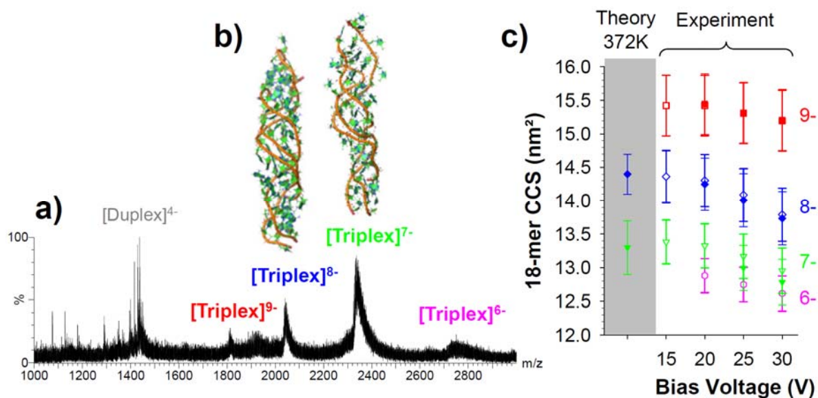
Figure 8: (a) ESI-MS spectra of the 18-mer triplex d(TC^+)_9 \cdot d(GA)_9 \cdot d(TC)_9 obtained from acidic conditions (150 mM NH_4OAc + acetic acid) at a bias voltage of 20 V on a Synapt HDMS ion mobility instrument. (b) Representative 3D structures obtained by MD in gas phase for the charge states 8- and 7-. (c) Agreement between theoretical and experimentally derived collision cross sections. Filled symbols: triplex with no ammonium adducts; open symbols: triplexes including the whole adduct distribution visible on the respective mass spectra. Adapted with permission from Arcella et al., J. Am. Chem. Soc., 2012, 134(15), pp 6596–6606. Copyright 2012 American Chemical Society.
