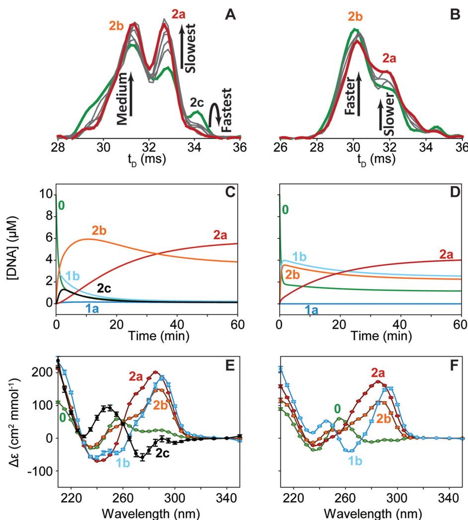
Figure 5. (A and B) Arrival time distribution in function of the time for the 4- charge state for the 2- K^+ stoichiometry at 500 \mu M KCl from green (3 min) to red (24h) through gray, respectively for 10 \mu M (A) 24TTG and (B) 23TAG. On each panel, arrival time distributions were area-normalized for visualization of the relative abundances. (C and D) Simulation of the concentrations of the species obtained using the best models at 500 \mu M KCl: (C) 0 \times ((1-2)/(1 \times (2|2))) for 24TTG and (D) 0 \times ((1-2)/(1-2)) for 23TAG. (E and F) Deconvoluted CD spectra for the ensembles defined by the kinetics model, respectively for (E) 24TTG and (F) 23TAG.
