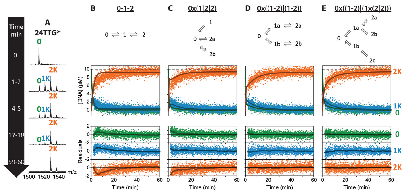
Figure 4. Kinetics of K^+ -binding (20°C) monitored by mass spectrometry of 10 \mu M 24TTG in 100 mM TMAA after adding KCl to reach a final concentration of 500 \mu M. (A) Mass spectra after addition of KCl at different time (integrated over 1 min accumulation). (B–E) Concentration of the complexes with 0, 1 or 2 potassium in green, blue and orange, respectively, as a function of time after K^+ addition. The data were fitted using the models described above each graph.
