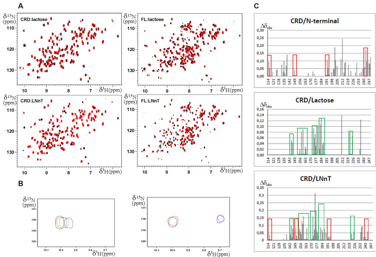
Figure 4. Complex formation involving Galectin-3. A] 15 N-HSQC spectra carried out on a 600 MHz NMR spectrometer equipped with a TCI cryoprobe at 300 K. Top left, free CRD at 40 μM concentration in black and CRD at 40 μM concentration in the presence of lactose at 1.5 mM in red; top right, free full length Galectin-3 (FL) at 30 μM concentration in black and FL at 30 μM concentration in the presence of lactose at 1.5 mM in red; bottom left, CRD at 40 μM concentration in black and CRD at 40 μM concentration in the presence of LNnT at 80 μM in red; bottom right, free full length Galectin-3 (FL) at 30 μM concentration in black and FL at 30 μM concentration in the presence of LNnT at 80 μM in red. B] Zoom in of HSQC: in left box, free CRD at 40 μM concentration in black and CRD at 40 μM concentration in the presence of lactose at 0.1 mM in red, 0.8 mM in green and 1.5 mM in blue; in the right box, CRD at 40 μM concentration in black and CRD at 40 μM concentration in the presence of LNnT at 28 μM in red and 90 μM in blue. C] Chemical shift variations observed on Galectin-3 CRD NH, top, induced by the N-terminal domain within FL (Table S2); center, induced by lactose (Table S3); bottom, induced by LNnT (Table S4). Values shown were calculated using the equation \Delta\delta_{obs} = [(\Delta\delta_{HN}^2 + \Delta\delta_N^2/25)]^{1/2} . In green boxes are highlighted residues affected by lactose. In red boxes are highlighted residues affected by the N-terminal domain within the full length protein.
