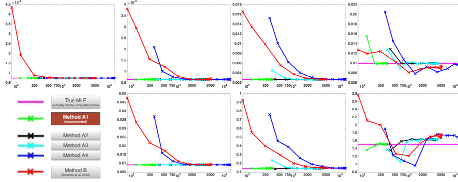
Fig. 1. Performance curves. MSE variations as a function of computation time (in sec). 1st row, \hat{\mathbf{w}} ; 2nd row, \hat{\mathbf{D}} . Columns match areas 0F, 1F, 2F, 3F from left to right.
