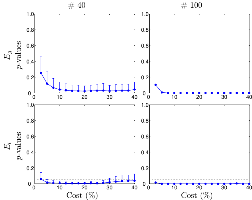
Figure 9: Comparison between the reliability of 40 and 100 subjects using the parcellation of 459 regions. Two global network parameters (Global and local efficiency) are compared. E_g (first row) and E_l (second row) p -values; on the left, 40 subjects (1000 bootstraps) and 100 subjects on the right. Results computed for cost from 2.5 to 40%. This figure can be compared to the first row of Fig. 4.
