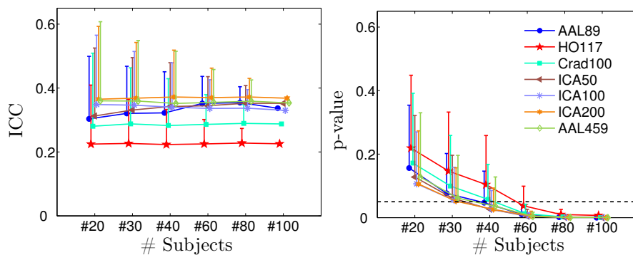
Figure 11: ICCs and their p-values for different parcellation templates and different number of subjects. Results are shown for betweenness centrality ( B ) at 1200tp and 20% cost.
