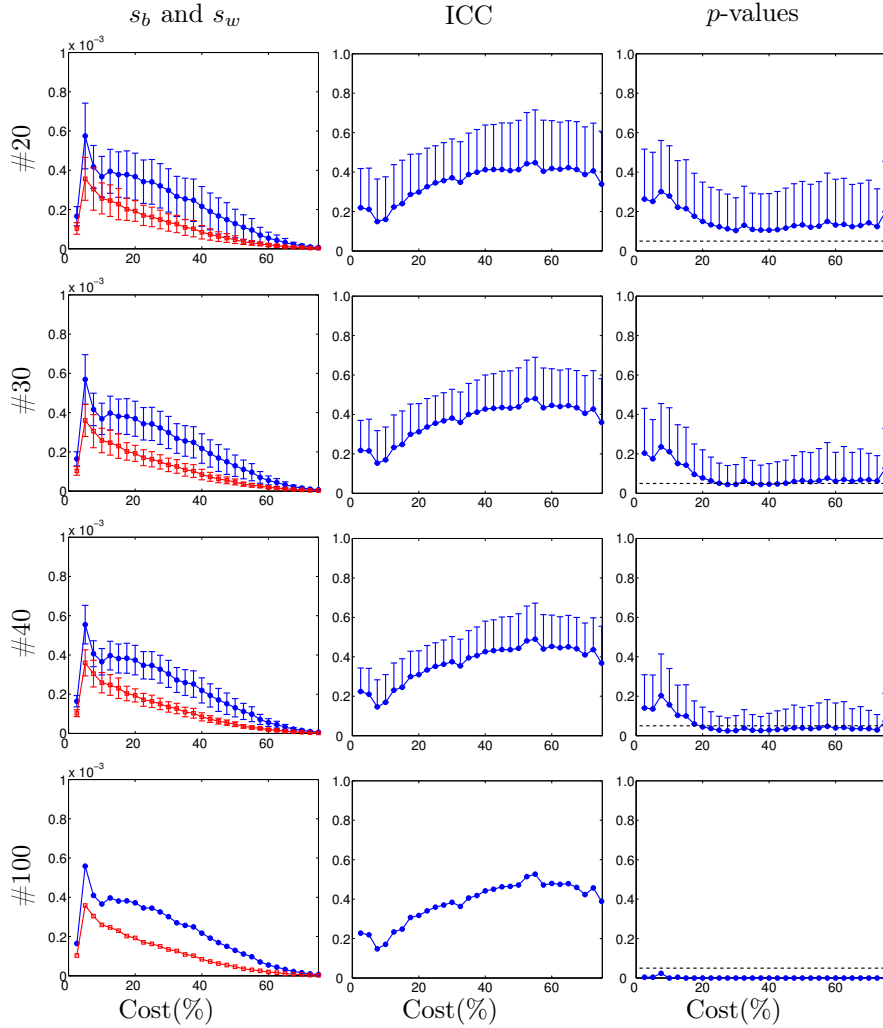
Figure 1: Reliability measures using ICC for global efficiency ( E_g ) and AAL89 as parcellation scheme. Each curve represents the between and within subjects variance (first column, respectively s_b in blue and s_w in red), values of ICC (second column) and associated p -values (third column) for E_g at 1200 time points as a function of the cost from 2.5% to 75%, in steps of 2.5%. Each row represents a different number of subjects (20, 30, 40 and 100 subjects). Error bars indicate one standard deviation of the bootstrap procedure. 1000 bootstraps were computed to select different subsamples of 20, 30 and 40 subjects. As the number of subjects is increasing, the p -values are decreasing, and the reliability is increasing. For 20 subjects, no p -values are significant, showing a poor reliability. However, for 40 subjects, p -values are significant for a large range of cost and reliable results are expected.
