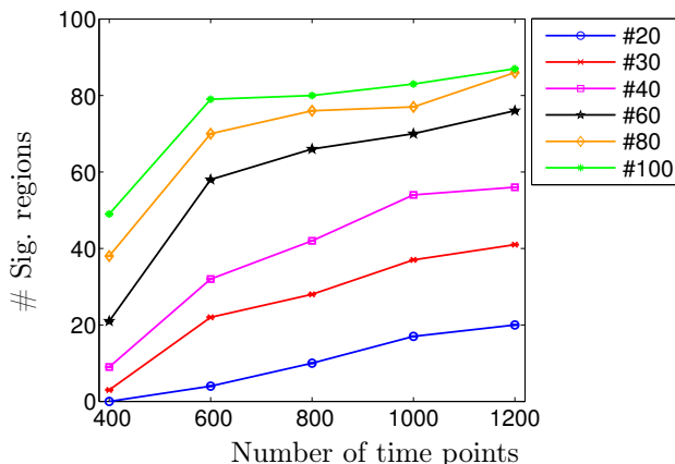
Figure 6: Reliability at the regional level using global efficiency and AAL89 parcellation scheme. Number of significant regions, computed using e_{g_i} , as function of the points in time for different number of subjects (corrected for multiple comparisons using a false discovery rate procedures at 0.05%). All the results shown are computed at 20% cost. The correspondence between scan duration and time points is as follows: 400 time points (4 min 48 s), 600 time points (7 min 12 s), 800 time points (9 min 36 s), 1000 time points (12 min 00 s) and 1200 time points (14 min 24 s). All the subdivisions were extracted from the beginning of the time series up to each threshold.
