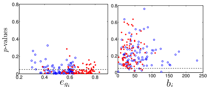
Figure 8: Reliability of brain regions in terms of cost using AAL89 as parcellation scheme. Mean e_{g_i} (left) and b_i (right) with their mean p -values. Computed for 40 subjects, 20% cost (in blue), 40% cost (in red) with 100 bootstraps (error bars are not shown) at 1200 points in time. Interestingly, the number of significant reliable regions obtained with betweenness is less than the one obtained with global efficiency. This may show that global efficiency is better at characterizing reliable hubs.
