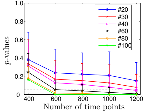
Figure 3: Reliability trade-off between number of subject and number of points in time using AAL89 as parcellation scheme. Evolution of the significance of global efficiency at global network level when increasing the number of points in time and the number of subjects. E_g mean p -values at different points in time applying 1000 bootstraps of 20, 30, 40, 60 and 80 subjects and for 100 subjects. All the results shown are computed at 20% cost. The number of subjects to achieve reliable results depends on the number of time points: a larger number of subjects is needed for a short scan duration. The correspondence between scan duration and time points is as follows: 400 time points (4 min 48 s), 600 time points (7 min 12 s), 800 time points (9 min 36 s), 1000 time points (12 min 00 s) and 1200 time points (14 min 24 s). All the subdivisions were extracted from the beginning of the time series up to each threshold.
