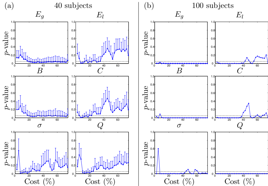
Figure 4: Reliability evaluation of different metrics using AAL89 as parcellation scheme. Mean p -values of ICC and standard deviation of 6 different global network parameters: global efficiency ( E_g ), local efficiency ( E_l ), betweenness centrality ( B ), clustering ( C ), small worldness ( \sigma ) and modularity ( Q ). Cost ranges from 2.5 to 75%. (a) 1000 bootstraps with 40 subjects randomly selected are shown using error bars with one standard deviation; (b) with 100 subjects.
