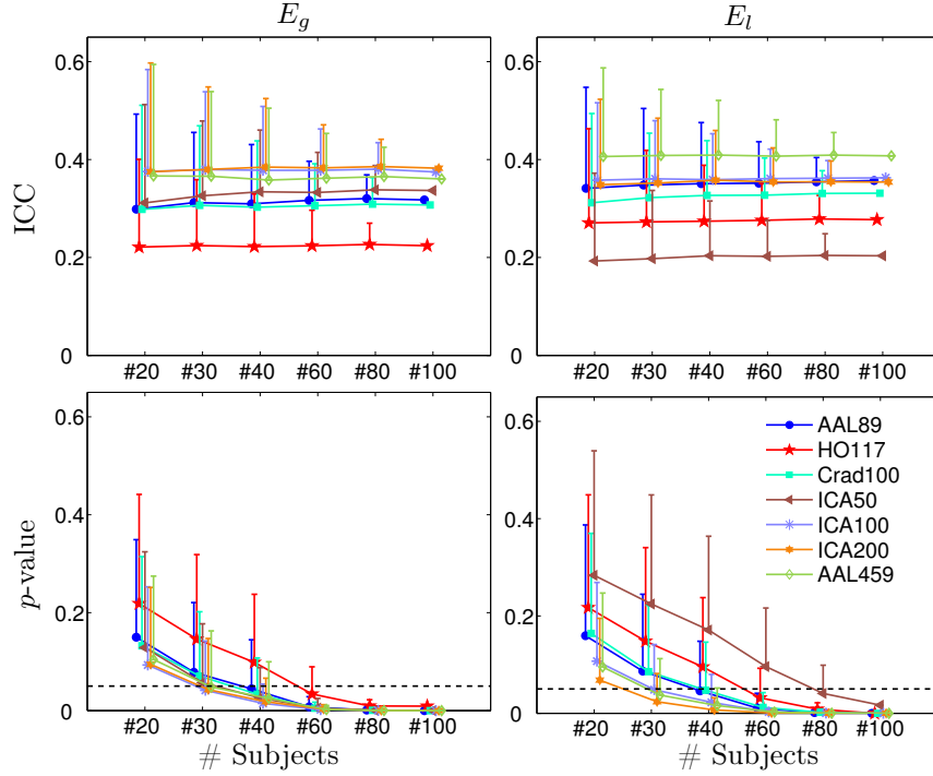
Figure 10: ICCs and their p-values for different parcellation templates and different number of subjects. Results are shown for global efficiency ( E_g ) and local efficiency ( E_l ) in first and second column, respectively, at 1200tp and 20% cost.
