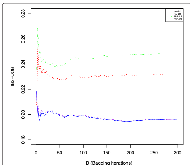
Fig. 15 Out Of Bag Integrated Brier Score evolution with the number of Bagging iterations: NA-LR and BRE-LR represents the adjusted Logrank splitting method with the Nelson-Aalen and the Breslow estimates respectively; NA-R2 and BRE-R2 are obtained using the Pseudo-R2 splitting method
