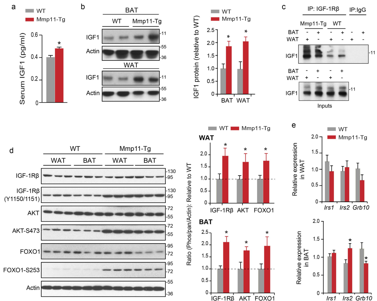
Figure 4. MMP11 activates the IGF1/AKT/FOXO1 axis. (a) Circulating IGF1 levels in Mmp11-Tg mice and controls ( n = 8/\text{group} ); (b) Immunoblots describing the expression of IGF1 in the WAT and BAT of Mmp11-Tg mice and controls; (c) Increased physical interaction between IGF1 and its receptor IGF1R \beta in the WAT and BAT of Mmp11-Tg compared to WT mice. Protein extracts were immunoprecipitated with an IGF1R \beta antibody and the interaction was revealed with an anti-IGF1 antibody; (d) left panel: Immunoblots for proteins involved in the IGF1 signalling pathway in the WAT and BAT of Mmp11-Tg mice compared to WT, right panel: quantification of the ratios of phosphorylated IGF1R \beta , pAKT, and pFOXO1 proteins relative to IGF1R \beta , AKT, and FOXO1, respectively, normalized to actin expression (data are presented as fold change of Mmp11-Tg values to WT values); (e) Expression profile of genes involved in the insulin/IGF1 pathway in the WAT and BAT of Mmp11-Tg and WT mice ( n = 6\text{--}7/\text{group} ).
