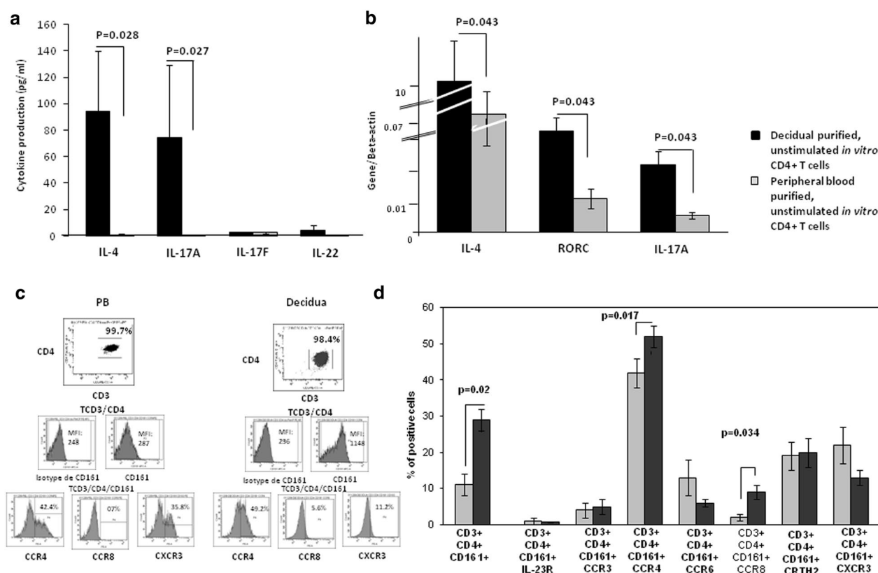
Fig. 1 Associated spontaneous production of both IL-17A and IL-4 and expression of CD161, CCR8 and CCR4 by fresh decidual CD3+CD4+ T cells in successful pregnancy. a Unstimulated decidual and PB CD4+ T cells purified from the same 9 pregnant women were cultured for 24 h and IL-4, IL-17A, IL-17F and IL-22 production (mean \pm SEM) was measured. b RT-PCR of unstimulated decidual and PB CD4+ T cells purified from the same 3 pregnant women for IL-17A, IL-4 and RORC was performed. c, d Th1 cells express CXCR3, whereas Th2 cells express CCR4, CCR8 and CRTH2 and Th17 cells express CD161, IL-23 receptor (IL-23R) CCR6 and CCR4. The associated expression of molecules expressed by Th17 cells and by Th1 and Th2 cells in fresh unstimulated CD4+ T cells purified from decidual and PB of the same pregnant women were analyzed by 4-color (CD3, CD4, CD161 and CCR4 or CCR8 or CXCR3) flow cytometry. c is a representative experiment and d data are represented as mean \pm SEM. For a, b and d the statistical analysis was performed with Wilcoxon test
