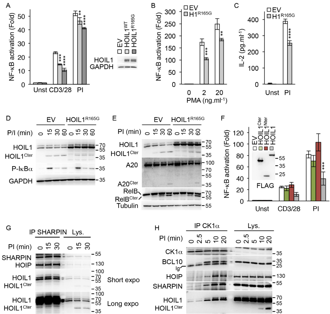
Fig. 3. HOIL1 cleavage participates in the optimal activation of NF-κB. (A) NF-κB reporter luciferase assay (mean±s.e.m.; n=3) of cells transfected with 10 μg of plasmids encoding for HOIL1 WT , HOIL1 R165G or with an empty vector (EV). Cells were stimulated with 0.5 μg ml -1 anti-CD3 plus anti-CD28 (CD3/28), or with 20 ng ml -1 PMA plus 300 ng ml -1 ionomycin (PI or P/I). The inset panel shows the expression of the plasmids when overexpressed in HEK293T cells. Unst, unstimulated. **P<0.01; ***P<0.001; ****P<0.0001 (ANOVA). (B) NF-κB luciferase assay (mean±s.e.m. of triplicate experiments) of Jurkat cells stably expressing HOIL1 R165G or an empty vector (EV), and stimulated with 0-20 ng ml -1 PMA plus 300 ng ml -1 ionomycin (PI). **P<0.01; ***P<0.001 (ANOVA). (C) Cells as in B were stimulated for 16 h. IL-2 secretion in the culture supernatants was determined by ELISA. Shown is the mean±s.e.m. of triplicate experiments. ****P<0.0001 (ANOVA). (D,E) Immunoblots of cells as in B. In E, cells were pretreated with 25 μM of the proteasome inhibitor MG132 for 30 min prior to stimulation. (F) NF-κB luciferase assay (mean±s.e.m.; n=5; ***P<0.001 by ANOVA) of Jurkat cells transfected with the indicated FLAG-tagged plasmids. Cells were stimulated as in A. The inset panel shows the expression of the constructs when overexpressed in HEK293T cells. (G,H) Jurkat lymphocytes were stimulated as in A. Cell lysates were immunoprecipitated (IP) with antibodies to SHARPIN (G) or to CK1α (H), and immunoblotting was performed as indicated. Lys., lysates; lg, light chain immunoblogulin. The positions of molecular mass markers (kDa) are shown. Data are representative of three independent experiments.
