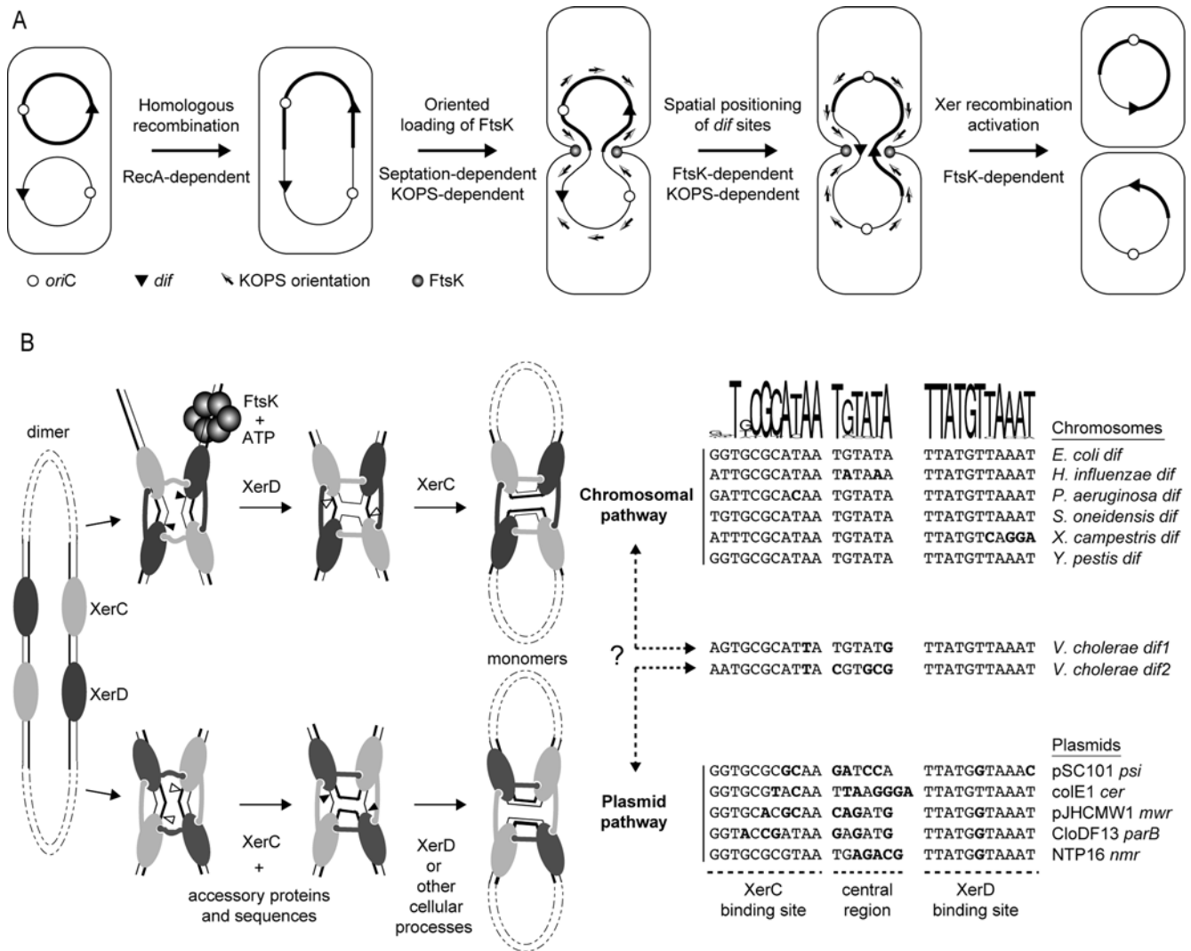
Figure 1. FtsK-dependent and FtsK-independent Xer recombination. A. Chromosome dimer formation and resolution in E. coli . The two homologous chromosomes are depicted by thick and thin lines, to allow for the visualization of crossovers. B. Link between the central region of XerCD-target sites (right) and the recombination pathway adopted at these sites (left). The XerCD- dif recombination complex is viewed from the C-terminal side of the recombinases, to show the C-terminal interactions of XerC and XerD. Strands cleaved by XerC and XerD in E. coli are shown with thick and thin lines, respectively. Positions of strand cleavages by E. coli XerC and XerD are indicated by white and black triangles, respectively. The WebLogo was generated using the alignment of putative dif sites from the larger chromosome of 27 \gamma -Proteobacteria (Text S1). The XerC-binding site, XerD-binding site and central region of dif FC are indicated below the alignment. doi:10.1371/journal.pgen.1000201.g001
