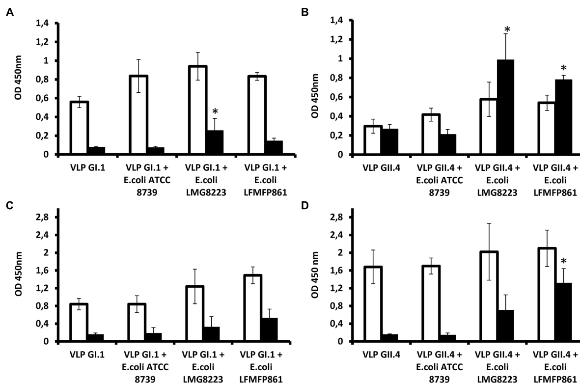
FIGURE 2 | Protection of histo-blood group antigen (HBGA) expressing bacteria on human norovirus (NoV) virus-like particles (VLPs) toward heat treatment. (A,B) Antigenicity detection of NoV GI.1 and GII.4 in the absence of bacteria, in the presence of non-HBGA expressing E. coli ATCC8739 or HBGA-expressing E. coli LMG8223 and LFMFP861 before (white bars) or after (black bars) heat treatment at 90°C for 2 min. (C,D) Mucin-binding
