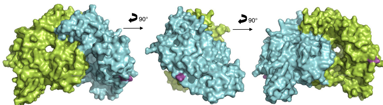
Fig. 4 Representation of solvent-accessible surface area of eNOS3 homodimer oxygenase domains (PDB :1M9M). Chain A and B are in green and cyan respectively. Glu298 is coloured in magenta in both chains
