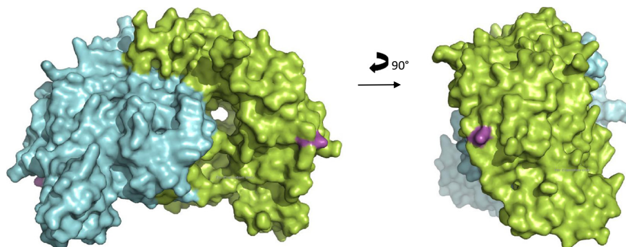
Fig. 5 NOS3 Glu298 [1m9m]
