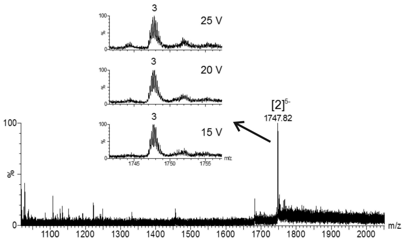
Figure 2. Electrospray mass spectrum of (AGG) 4 A in the presence 150 mM ammonium acetate. The final single strand RNA concentration was 18 \mu M. 10% v/v of methanol was added 1 h before measurement. The peak annotation [n]^z indicates the number of strands ( n ) and the total charge ( z ). The distribution of the number of ammonium ions preserved in the structure is shown in the inset. The distribution is presented at three bias voltages.
