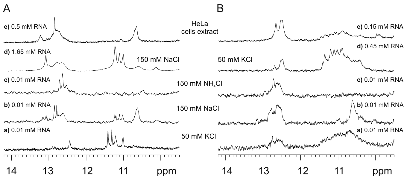
Figure 5. Imino regions of the ^1\text{H} NMR spectra of (A) \text{G}(\text{CGG})_2\text{C} and (B) \text{G}(\text{CGG})_4\text{C} at 10^\circ\text{C} in the presence of (Aa, Ba, Ad, Bd) 50 mM KCl, 10 mM potassium phosphate and 0.1 mM EDTA, pH 6.8, (Ab, Bb) 150 mM NaCl, 10 mM sodium phosphate, 0.1 mM EDTA, pH 6.8, (Ac, Bc) 150 mM \text{NH}_4\text{Cl} , 10 mM Tris/HCl, 0.1 mM EDTA, pH 6.8 and (Ae, Be) HeLa cell extract. The poor S/N ratio observed for \text{G}(\text{CGG})_4\text{C} is due to polymorphism or/and the presence of higher order structures.
