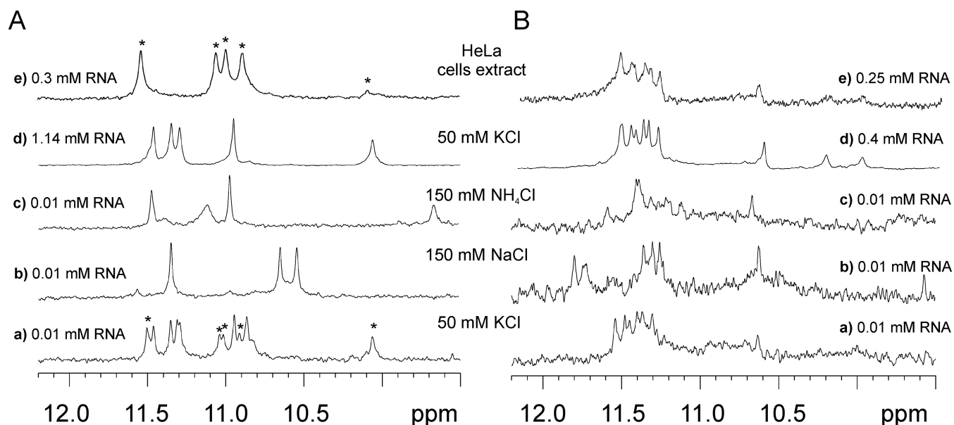
Figure 3. Imino region of the ^1\text{H} NMR spectra of (A) (AGG) 2 A and (B) (AGG) 4 A at 25°C in the presence of 50 mM KCl, 10 mM potassium phosphate and 0.1 mM EDTA, pH 6.8 (Aa, Ba, Ad, Bd), 150 mM NaCl, 10 mM sodium phosphate, 0.1 mM EDTA, pH 6.8 (Ab, Bb), 150 mM NH 4 Cl, 10 mM Tris/HCl, 0.1 mM EDTA, pH 6.8 (Ac, Bc) and the HeLa cell extract (Ae, Be). The poor S/N ratio observed for (AGG) 4 A is due to polymorphism or/and the presence of higher order structures.
