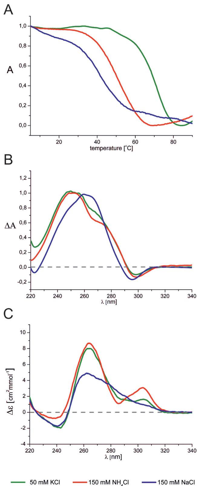
Figure 1. (A) Normalized UV melting profiles of (AGG) 4 A at 295 nm, (B) normalized thermal differential spectra of (AGG) 2 A and (C) CD spectra of (AGG) 2 A at 25°C. All the spectra were recorded in the presence of 50 mM KCl, 10 mM potassium phosphate and 0.1 mM EDTA, pH 6.8 (green), 150 mM NH 4 Cl, 10 mM Tris/HCl, 0.1 mM EDTA, pH 6.8 (red) and 150 mM NaCl, 10 mM sodium phosphate, 0.1 mM EDTA, pH 6.8 (blue).
