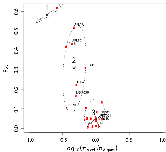
Fig 1. Population genetic parameters partition Anopheles coluzzii and A. gambiae candidate genes into discrete clusters. For 26 genes sequenced from wild A. coluzzii and A. gambiae mosquitoes from Burkina Faso, scatterplot indicates the log-ratio of nucleotide diversity, \pi , for A. coluzzii / A. gambiae (x-axis) and pairwise F_{st} between A. coluzzii and A. gambiae (y-axis). Negative values for log-ratio of \pi indicate greater diversity in A. gambiae positive values greater diversity in A. coluzzii , and a value of 0 indicates no difference in nucleotide diversity between A. coluzzii and A. gambiae . The names of genes subsequently tested by functional analyses are shown, for others see S1 Table. Dashed ovals indicate unbiased hierarchical clusters identified by the method of Ward based on minimized within-cluster variance, with optimal number of clusters k = 3 as determined by the Krzanowski-Lai index (S1 Fig), stars indicate cluster centroids. d pairwise F_{st} between A. coluzzii and A. gambiae . Negative values for log-ratio of \pi indicate greater diversity in A. gambiae positive values greater diversity in A. coluzzii , and a value of 0 indicates no difference in nucleotide diversity between A. coluzzii and A. gambiae . The names of genes subsequently tested by functional analyses are shown, for others see S1 Table. Dashed ovals indicate unbiased hierarchical clusters identified by the method of Ward based on minimized within-cluster variance, with optimal number of clusters k = 3 as determined by the Krzanowski-Lai index (S1 Fig), stars indicate cluster centroids.
