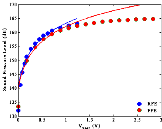
Figure 1: Sound pressure level (dB) at the surface of the breast phantom at the output of the waveguide versus the applied root mean square voltage V_{RMS} for RFE acquisitions (blue dots) and FFE acquisitions (red dots). The lines are the corresponding linear fits performed for 0 \leq V_{RMS} \leq 1 V.
