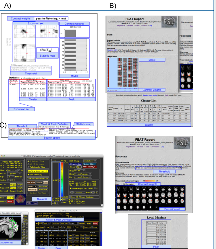
Fig. 2: Mapping between the information displayed as a summary of the results in A) SPM, B) FSL and C) AFNI and the corresponding entities in NIDM.
