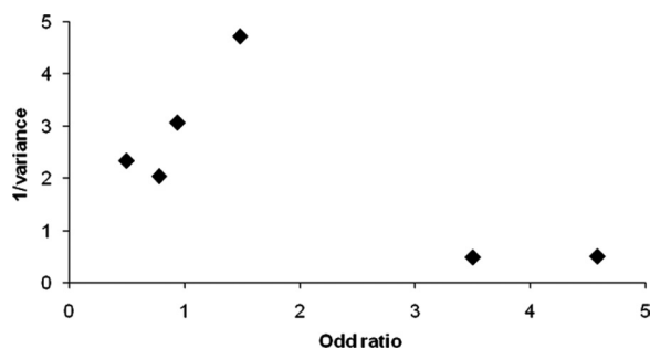
FIG. 3. Funnel plot of the studies of POC use and MI risk.
