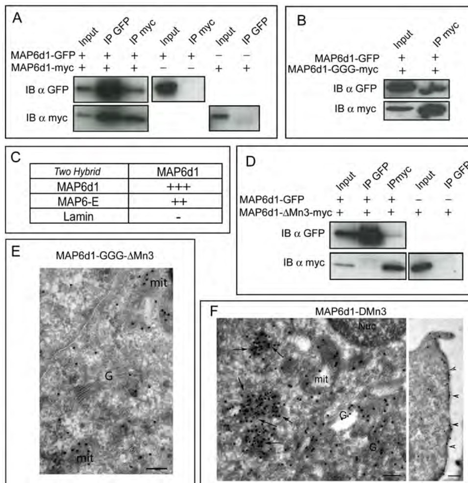
Fig. 7. MAP6d1 can multimerize. A, COS-7 cells overexpressing MAP6d1-GFP and MAP6d1-myc were lysed. Proteins were immunoprecipitated with antibodies against either GFP or myc, separated by SDS-PAGE and immunoblotted with each antibody. In the control experiments, COS-7 cells over-expressing either MAP6d1-myc or MAP6d1-GFP were lysed, and protein was immunoprecipitated with anti-GFP or anti-myc antibodies, respectively. B, MAP6d1 multimerization does not require cysteines. COS-7 cells overexpressing MAP6d1-GFP and MAP6d1-GGG-myc were lysed, and the proteins were immunoprecipitated as in A. Both proteins are present in the immunoprecipitate. C, Two-hybrid experiments to test the interactions between MAP6d1 and itself, MAP6-E or lamin. MAP6d1 interacts with itself and with MAP6-E. D, MAP6d1 multimerization requires the Mn3 module. COS-7 cells overexpressing MAP6d1-GFP and MAP6d1- \Delta Mn3-myc were lysed, and proteins were immunoprecipitated as in A. No co-immunoprecipitation was observed between MAP6d1 and MAP6d1- \Delta Mn3. E, NIH/3T3 cells were transfected with a plasmid encoding MAP6d1-GGG- \Delta Mn3-myc, and cryosections were labeled using an anti-myc antibody and immuno-gold. MAP6d1-GGG- \Delta Mn3 is not concentrated on the Golgi apparatus but is dispersed throughout the cytoplasm. Mitochondria are still heavily labeled, but no protein aggregates were observed. F, NIH/3T3 cells were transfected with a plasmid encoding the mutant MAP6d1- \Delta Mn3-myc and analysed as in E. MAP6d1- \Delta Mn3 associates with the Golgi, the plasma membrane (arrowheads) and cytoplasmic vesicles (arrows). G: Golgi apparatus; mit: mitochondria. Bars, 200 nm.
