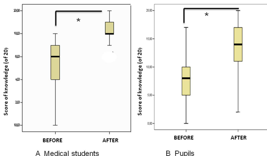
Figure 3 Knowledge evaluation: A: For Medical students before and after training course (maximum score of 20). P < 0.05 ; B: For Pupils before and after course (maximum score of 20) P < 0.05 .
