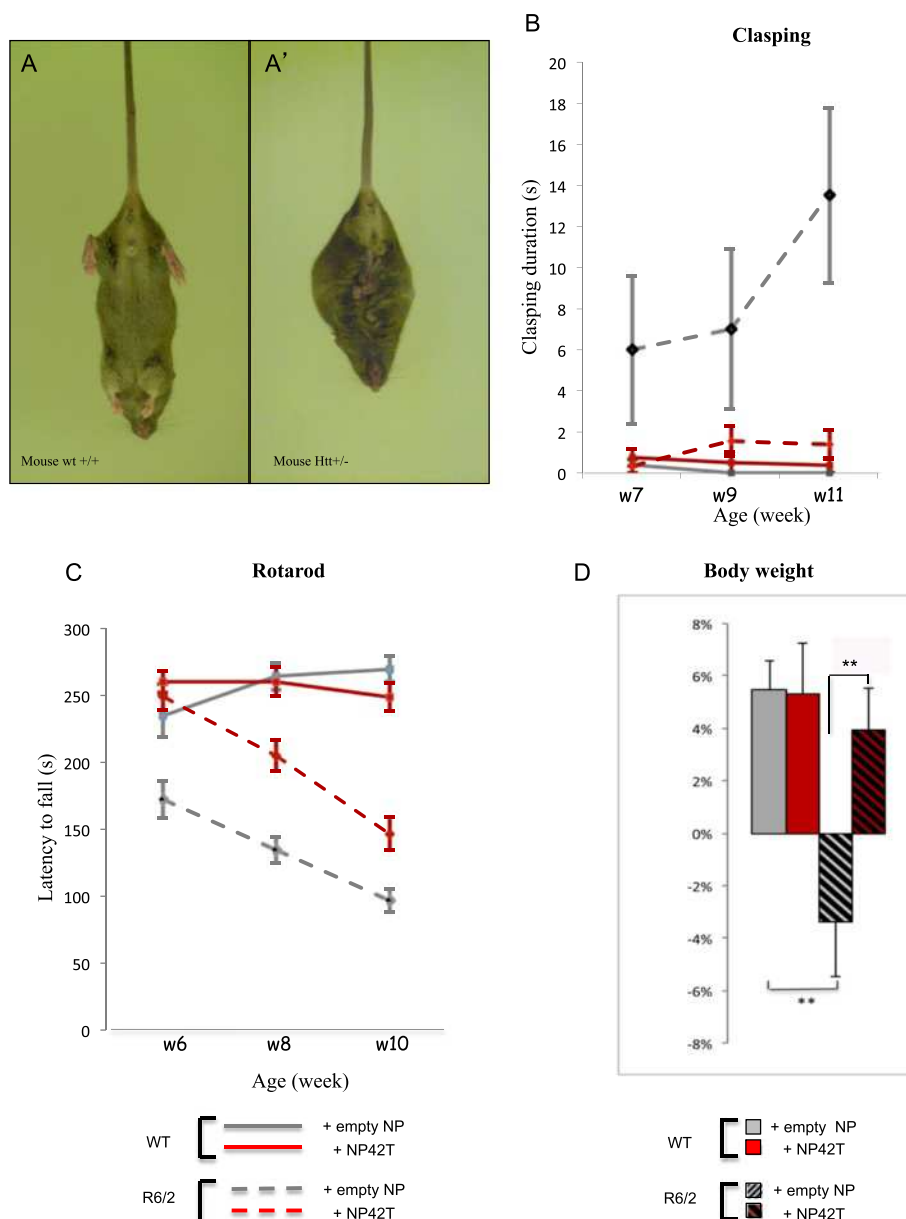
Figure 4 Aonys® NP42T treatment ameliorates behavioural deficits in R6/2 mice. (A) R6/2 mice present a foot-clasping behaviour ( A' ) absent in WT littermates ( A ). ( B ) Only groups treated with NP42T show a clear inhibition of clasping duration at 11wks: Two way ANOVA ( F(\text{Genotype} \times \text{Treatment})_{1,25} = 6.4, p = 0.0179 ). Post-hoc comparison (Bonferroni's test): **p < 0.01 WT (NP) vs R6/2 (NP); **p < 0.01 R6/2 (NP) vs R6/2 (NP42T), with two way ANOVA ( F(\text{Group} \times \text{Time})_{6,78} = 1.0, p = 0.4022 ) similar over time. ( C ) Rotarod performances of wild-type (WT) or R6/2 mice treated with NP42T or with empty NP (placebo) at 6, 8 and 10 weeks of age. Motor deficit is identified in R6/2 mice already at week6. Beneficial effect is observed for R6/2 treated with NP42T: Two way ANOVA ( F(\text{group} \times \text{time})_{6,78} = 2.362, p < 0.05 ) indicates that rotarod deficit of the four groups of mice was different over time. Post-hoc comparison (Bonferroni's test): 6wks *p < 0.05 R6/2 (NP) vs R6/2 (NP42T); *p < 0.05 ; 8wks ***p < 0.001 WT (NP) vs R6/2 (NP); *p < 0.05 R6/2 (NP) vs R6/2 (NP42T); 10wks ***p < 0.001 WT (NP) vs R6/2 (NP); ns R6/2 (NP) vs R6/2 (NP42T). ( D ) Body weight of R6/2 mice is recovered by both early and late administrations of NP42T. Body weight variations were measured in WT and R6/2 mice, treated with empty NP (placebo) or with NP42T. Graphs represent the body weight evolution from 8wks to 11wks in percentage. In HD mice, NP42T inverts the curves and restores a gain of weight in pre-symptomatic. One way ANOVA: ( F_{(3,24)} = 5.2, p < 0.01 ). Post-hoc comparison (Fisher's LSD): **p < 0.01 WT (NP) vs R6/2 (NP); **p < 0.01 R6/2 (NP) vs R6/2 (NP42T). Data represent means \pm SEM ( n = 5-9 per group).
