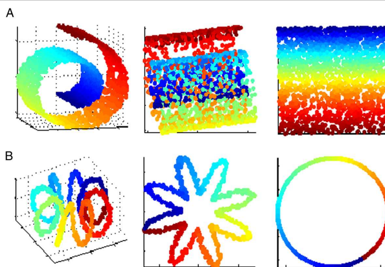
Figure 1 Reduction of two complex datasets A (a roll) and B (a helicoidal tore) with two methods, classical linear method (PCA) versus nonlinear method (ISOMAP). PCA relies on projections: original data (left) are represented in a three-dimensional space. PCA projected data into a two-dimensional space along their principal axes and the neighboring relationships are not preserved (center). ISOMAP properly unfolds the data while preserving true neighbors (right). True' neighbors are dots of similar colors: the dimensionality reduction technique does not respect neighboring relationships when a red dot lies next to a blue dot.
