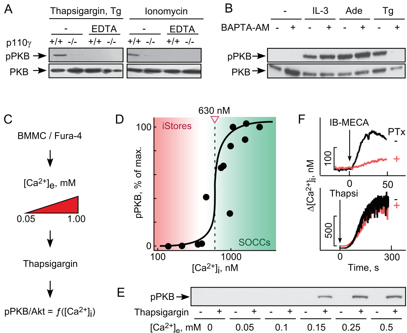
Figure 2. Thapsigargin-triggered PI3K \gamma activation requires influx of extracellular Ca 2+ . (A) Where indicated, IL-3 starved BMMCs were incubated with EDTA (5 mM) for 5 min, before cells were stimulated with thapsigargin (1 \mu M) or ionomycin (1 \mu M). Cells were lysed 5 min after stimulation, and phosphorylation of PKB/Akt on Ser473 was analyzed. (B) BMMCs as in (A) were pretreated for 10 min with the cell-permeable Ca 2+ -chelator BAPTA/AM (10 \mu M) and stimulated either with IL-3 (10 ng/ml), adenosine (1 \mu M), or thapsigargin (1 \mu M). (C, D) BMMCs were loaded with the ratiometric low affinity Ca 2+ probe Fura-4F/AM for 10 min in physiologic HEPES buffer at 1 mM Ca 2+ (for details see Text S1). After the loading, washed cells were resuspended in the presence of increasing Ca 2+ concentrations (extracellular Ca 2+ , [Ca 2+ ] e ) to modulate maximal stimulation-induced intracellular Ca 2+ levels ([Ca 2+ ] i ). Cells were then stimulated with 0.5 \mu M thapsigargin, and maximal [Ca 2+ ] i increase and phosphorylation of PKB/Akt were measured. pPKB S473 levels are displayed as a function of the individually determined [Ca 2+ ] i . Data points come from two independently performed experiments. (E) Representative anti-phospho-PKB/Akt immunoblot as used to determine pPKB/Akt levels in (D). (F) Intracellular Ca 2+ concentrations were measured in wild type BMMCs following stimulation with the adenosine 3A receptor-selective agonist N 6 -(3-iodobenzyl)-adenosine-5'- N -methylcarbox-amide (IB-MECA) (10 nM) or thapsigargin (1 \mu M). B. Pertussis toxin (100 ng/ml) was added 4 h before stimulation where marked. doi:10.1371/journal.pbio.1001587.g002
