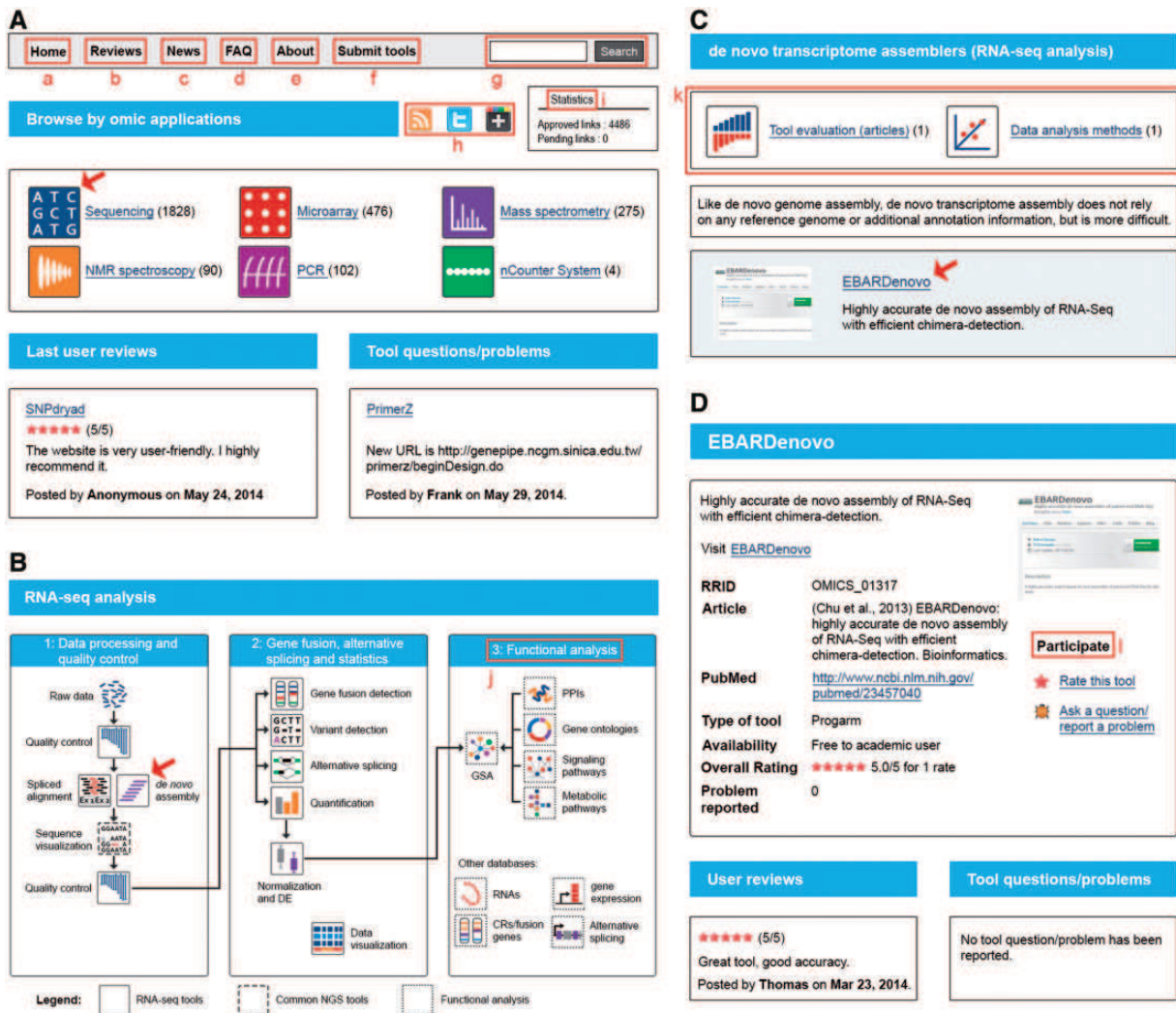
Figure 1. OMICtools structuration. (A) Classification by technologies. (B) Classification by analytical steps, as illustrated by RNA sequencing analysis. (C) List of tools for a given analytical step, as illustrated by de novo assembly (D) Tool description. Several features are highlighted. (a) Homepage button. (b) User reviews. (c) Latest tools added to the directory. (d) FAQ. (e) About us. (f) Link to the submission page. (g) Global site search bar. (h) Widgets that allow users to share this page with their social networks. (i) Statistics. (j) Associated databases. (k) Associated published evaluations of algorithm performance and data analysis methods. (l) Interface for interacting with the user community. Illustrated pages will be open by clicking on the icons indicated by the red arrows
