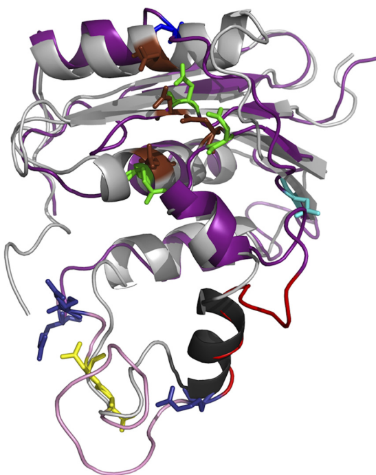
FIG 2 Cartoon representation of the superimposition of the E. coli RNase H structure and the HBV RNase H model. The E. coli experimental structure is gray, with the C-helix and catalytic residues as brown sticks. The HBV RNase H model is deep purple. The first three catalytic residues and the four D residue candidates for the 4th catalytic residue are shown in sticks and colored as in Fig. 1, i.e., green (D689, E718, and D737), yellow (D777 and D778), cyan (D807), and blue (D817; top of the model). The putative basic protrusion is shown in pink, with the C-helix in red and arginine residues in deep blue (bottom of the model).
