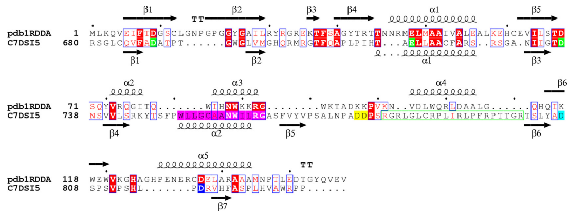
FIG 1 Pairwise sequence alignment of E. coli and HBV RNases H. The E. coli and HBV sequence are designated by pdb1RDDA and C7DSI5, respectively. Identical residues are shown in red boxes. Similar residues are in red letters. The first three catalytic residues of the HBV RNase H (D689, E718, and D737) are in green. The four D residue candidates for the 4th catalytic residue are in yellow (D777 and D778), cyan (D807), and blue (D817). The HBV RNase H putative C-helix is highlighted in magenta. The dots indicate gaps. Protein secondary structures deduced from the 3-D structure ( E. coli ) or predicted (HBV) are indicated above and below each sequence, respectively, with the numbering of each secondary structure element (e.g., \alpha 1 and \beta 1 ). The figure was generated with the ESPrpt server (50).
