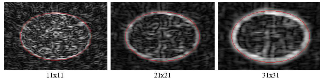
Figure 3: PZMI_{1,1} values estimated with a 11 \times 11 , 21 \times 21 and 31 \times 31 window size. In this figure only a rectangular window around the elliptic region of the simulated image is shown. The elliptic region boundary is shown in red.
