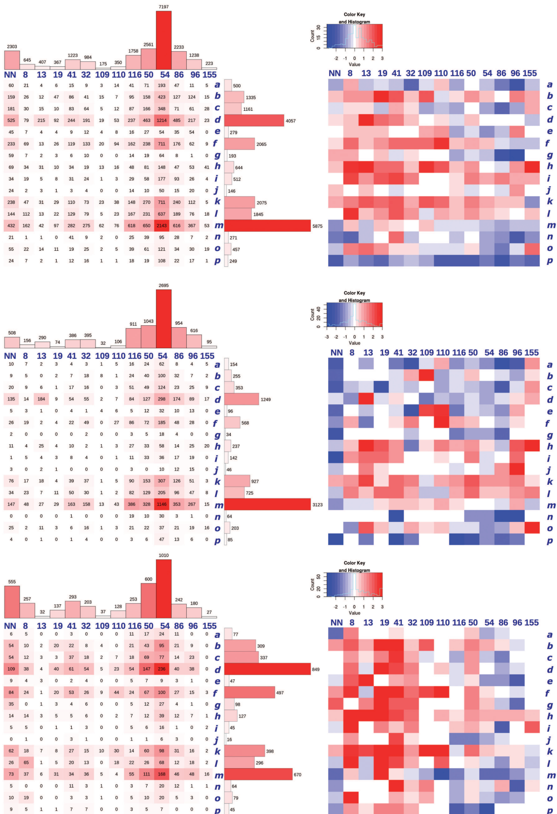
Figure 2. Interaction matrices for direct polar contacts of the three groups of structures with crystallographic resolution between 1.90 and 2.80 Å (bin R 2 ). Top: 636 protein/DNA complexes, Umb-R 2 . Center: 255 complexes of transcription factors, TrF-R 2 . Bottom: 101 complexes of nucleases, Nuc-R 2 . The matrices on the left show how many peptide blocks, PBs, interact with nucleotide conformers, ntCs, the highest populations are highlighted in red. The matrices on the right show how much are the interactions statistically different from their expected frequencies estimated by
