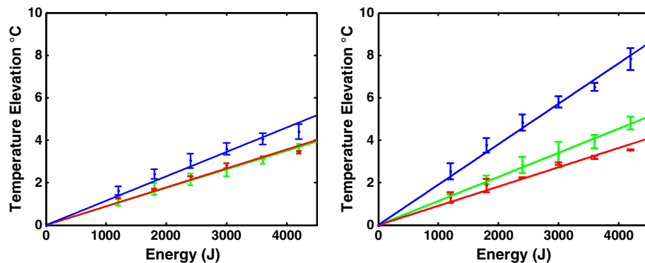
Figure 5 Temperature elevation as a function of energy. Measured heating using 220 kHz (left) and 710 kHz (right) in bare (blue), cap (green), and wig (red) skull setups. Standard deviation is displayed as error bars.
