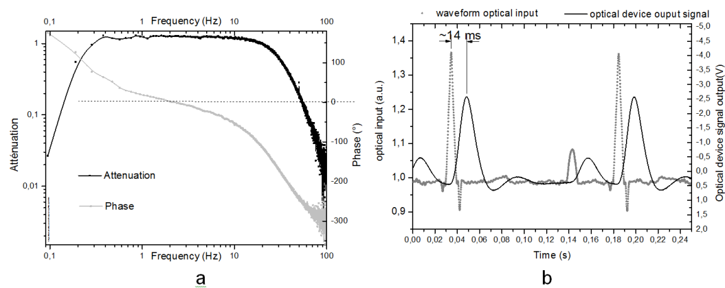
Fig. 3. (a) Bode diagram of the optical device. The band pass filter characteristics fit the expected attenuation specifications. (b) Optical device response to a typical ECG waveform excitation signal. At about 14 ms peak delay, a curve broadening can be noticed.
