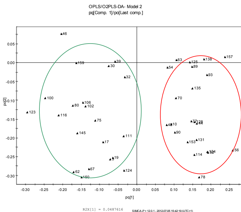
Fig. 3. pq loading plot of OPLS-DA model 2 (Table 1): scatter Plot of the X- and Y-loadings (p and q). This plot shows how the responses (Y's) varied in relation to each other, i.e. which provided similar information and their relationship to the terms of the model. Two tendencies could be seen. Peaks framed in red were higher levels in ASD urine, and peaks framed in green were lower.
