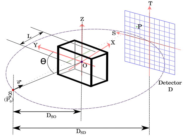
Fig. 1. Acquisition parameters of axial 3D cone-beam flat detector geometry.
