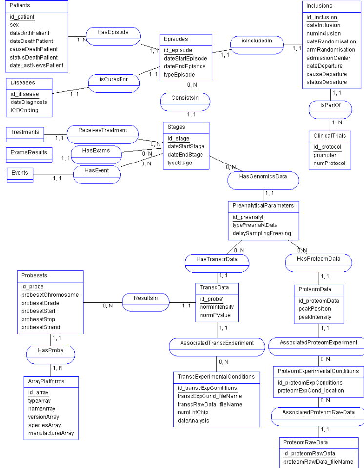
Figure 2: Data Modeling
