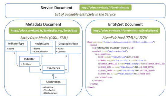
Figure 1 - OData service overview and OData Entity Data Model used for the FSN's data
