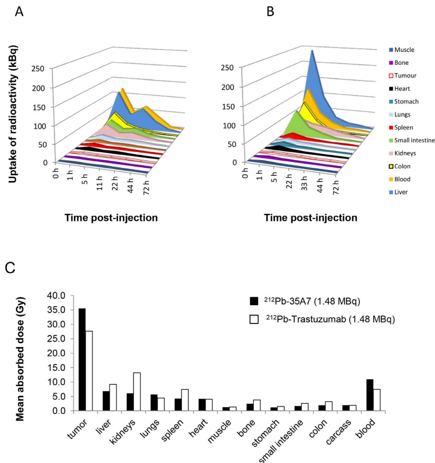
Figure 7. Uptake of radioactivity ( \text{UOR}_{\text{RIT}} ) per tissue (Bq) was determined using the values obtained during biodistribution experiments (Figure 6). (A) ^{212}\text{Pb} -35A7 (anti-CEA). (B) ^{212}\text{Pb} -Trastuzumab (anti-HER2). (C) Mean absorbed doses for ^{212}\text{Pb} -35A7 and ^{212}\text{Pb} -Trastuzumab. The total cumulative decay per tissue ( \bar{A}_{\text{TS}} ) was calculated from the area under each \text{UOR}_{\text{RIT}} curve and multiplied by 8.7 MeV (the mean energy emitted at each decay of ^{212}\text{Pb} and daughters). The ratio between tumor absorbed dose and blood absorbed dose was 3.2 ( ^{212}\text{Pb} -35A7) and 3.7 ( ^{212}\text{Pb} -Trastuzumab). The tumor-to-organ absorbed doses ratio were 5.2 (liver) and 5.8 (kidney) for ^{212}\text{Pb} -35A7 and 3.0 (liver) and 2.1 (kidney) for ^{212}\text{Pb} -Trastuzumab.
