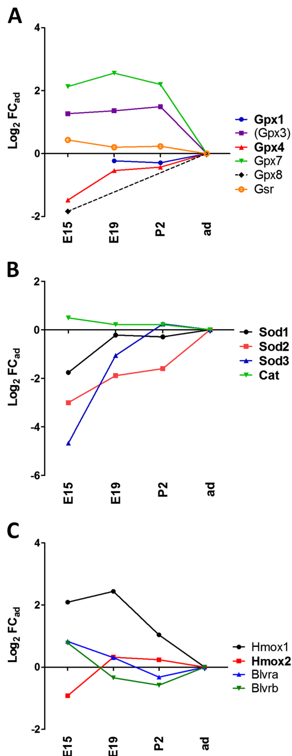
Figure 5 Developmental profiles of other antioxidant enzymes. (A) shows gene expression profiles for different glutathione peroxidases and glutathione reductase, (B) shows gene expression profiles for superoxide dismutases and for catalase, and (C) for heme oxygenases and biliverdin reductases. Abbreviations, data analysis, and data expression as in Figures 2 and 3.
