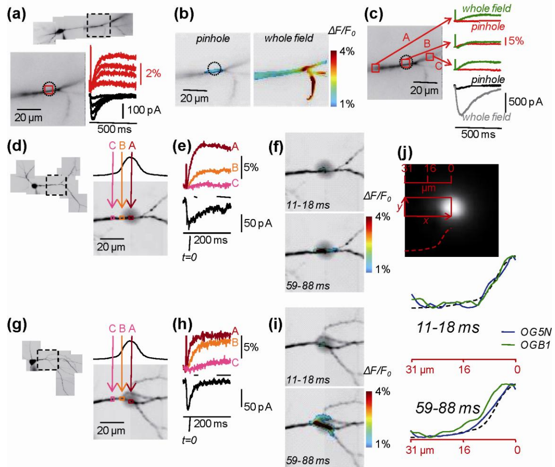
Figure 2: Simultaneous photolysis and \text{Ca}^{2+} imaging. (a) Reconstruction of a hippocampal neuron filled with 500 \mu\text{M} OG5N; in the recording position image below the UV spot (150 \mu\text{m} pinhole) represented by a dotted circle; red and black traces are respectively the \Delta F/F_0 \text{Ca}^{2+} signals in the red square and the somatic currents associated with UV flashes of 1, 2, 3 and 4 ms uncaging glutamate. (b) Spatial distributions of \Delta F/F_0 superimposed to the image represented in a colour scale during the period of 150-200 ms after a 3 ms pinhole UV flash (left) and after a 0.2 ms whole field UV flash (right). (c) \Delta F/F_0 signals after the pinhole UV flash (red traces) and after the whole field UV flash (green traces) in the three regions A-C indicated on the left image; correspondent somatic currents indicated below. (d) Reconstruction of a cultured hippocampal neuron filled with 500 \mu\text{M} OG5N; in the recording position image on the right the position of the UV spot (200 \mu\text{m} pinhole) is represented by a gray shadow; the coloured frames indicate three regions of interest (A, B and C) in the middle of the spot, in the periphery and outside the spot. (e) \Delta F/F_0 associated with a UV flash (occurring at t=0 ) uncaging NMDA from the regions A-C in d; somatic recording of the NMDA current below (black
