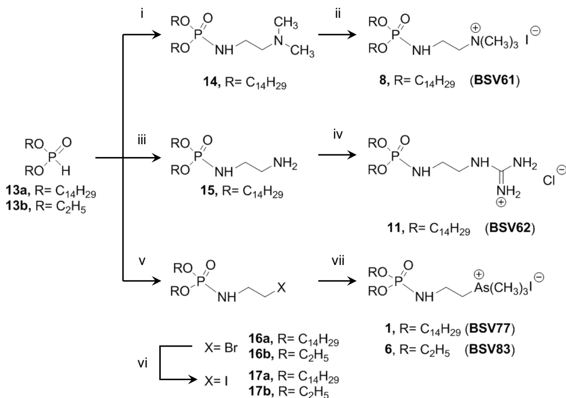
Figure 2. Reaction scheme for the synthesis of cationic lipids 1 , 6 , 8 , and 11 . Reagents and conditions: (i) \text{H}_2\text{N}(\text{CH}_2)_2\text{N}(\text{CH}_3)_2 , \text{CBrCl}_3 , DIPEA, \text{CH}_2\text{Cl}_2 , 0\text{ }^\circ\text{C} for 1 h then RT for 5 h, 85%. (ii) \text{CH}_3\text{I} , \text{CH}_2\text{Cl}_2 , reflux, O/N, 92%. (iii) \text{H}_2\text{N}(\text{CH}_2)_2\text{NH}_2 , \text{CBrCl}_3 , DIPEA, \text{CH}_2\text{Cl}_2 , 0\text{ }^\circ\text{C} for 1 h then RT for 5 h, 85%. (iv) 1H -pyrazole-1-carboxamide hydrochloride, EtOH, reflux, O/N, 88%. (v) \text{HBr}\cdot\text{H}_2\text{N}(\text{CH}_2)_2\text{Br} , \text{CBrCl}_3 , DIPEA, \text{CH}_2\text{Cl}_2 , 0\text{ }^\circ\text{C} for 1 h then RT for 3 h, 90% for \text{R}=\text{C}_{14}\text{H}_{29} and 95% for \text{R}=\text{C}_2\text{H}_5 . (vi) \text{NaI} , THF, reflux, O/N, 72% for \text{R}=\text{C}_{14}\text{H}_{29} and 82% for \text{R}=\text{C}_2\text{H}_5 . (vii) \text{AsMe}_3 , THF, 60\text{ }^\circ\text{C} for 48 h, 82% for \text{R}=\text{C}_{14}\text{H}_{29} and 73% for \text{R}=\text{C}_2\text{H}_5 .
