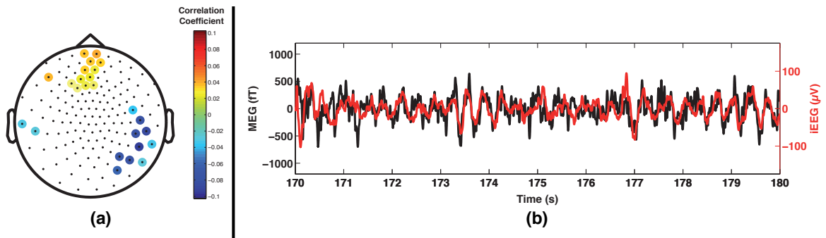
Figure 2: (a) Zero-lag correlation of a right hippocampus electrode with the MEG sensor array is shown as an MEG scalp topography. Sensors with peak correlations at non-zero lag are masked to eliminate spurious correlations due to neural connectivity rather than volume conduction. (b) In this trace, spontaneous theta oscillations are visible with zero-lag synchrony in the hippocampus depth electrode recording and the most correlated MEG sensor.
