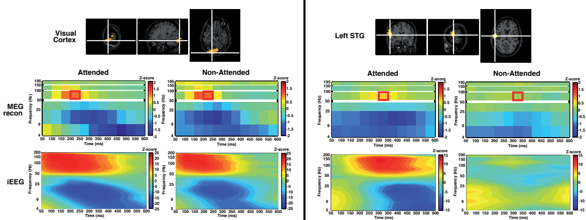
Figure 1: Spectral modulations derived from MEG source reconstruction compared favorably to those derived from intracranial EEG data. At left, the MEG reconstruction for a visual cortex source and the time-frequency map from the nearest intracranial EEG electrode, with power modulations up to 100 Hz detected with both techniques in both conditions. At right, the activity from left superior temporal gyrus (STG), showing task modulation of high gamma activity with both MEG source reconstruction and intracranial EEG. For each location, the activation maps superimposed on the structural MRI slices correspond to the MEG power modulation over the time-frequency window indicated by the red box on the MEG spectrogram.
