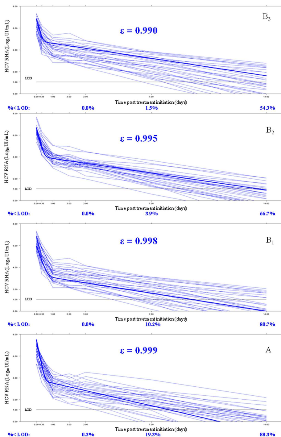
Figure 1 Time course of log 10 HCV RNA after treatment initiation for one simulated dataset with one design (N = 30 patients per PI and n = 7 viral load measurements). A : assuming \epsilon = 0.999 ; B 1 : assuming \epsilon = 0.998 ; B 2 : assuming \epsilon = 0.995 ; B 3 : assuming \epsilon = 0.990 . In bold, the mean curves predicted by the mean parameters of the model. LOD: limit of detection = \log_{10}(12) \approx 1.08 \log_{10} IU/mL; % < LOD: percentage of patients below the LOD at day 3, 7 and 14 estimated from 500 simulated datasets. The mean 14 days log drop were 6.56 log 10 IU/mL with \epsilon = 0.999 , 6.25 log 10 IU/mL with \epsilon = 0.998 , 5.85 log 10 IU/mL with \epsilon = 0.995 and 5.52 log 10 IU/mL with \epsilon = 0.990 .
