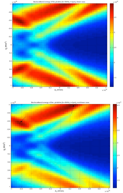
Figure 3 : Energy of the backscatter at different modulation indices \beta_1 and \beta_2 the (top image) shows the linear response of the micro-bubbles and the (bottom image) shows the non-linear response.
