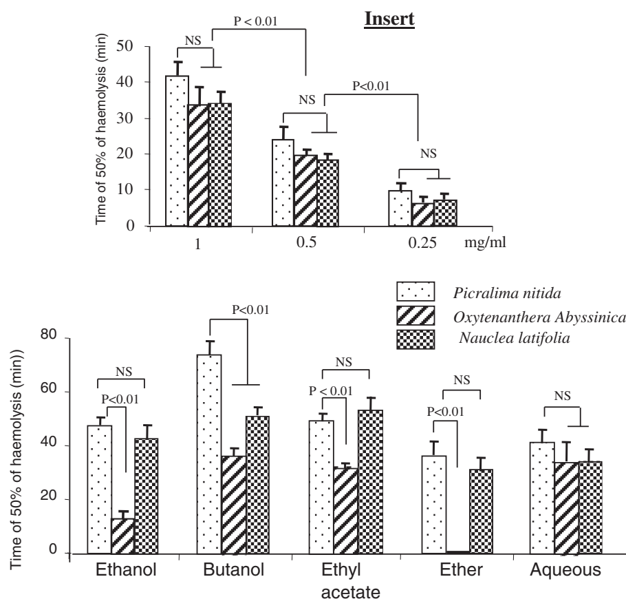
Figure 3 Antioxidant capacity of plant extracts. Antioxidant capacity of plant extracts was determined in a solution of 1 mg/ml as described in the Materials and Methods section. Results are mean \pm SEM. Each value represents the mean of three determinations.
