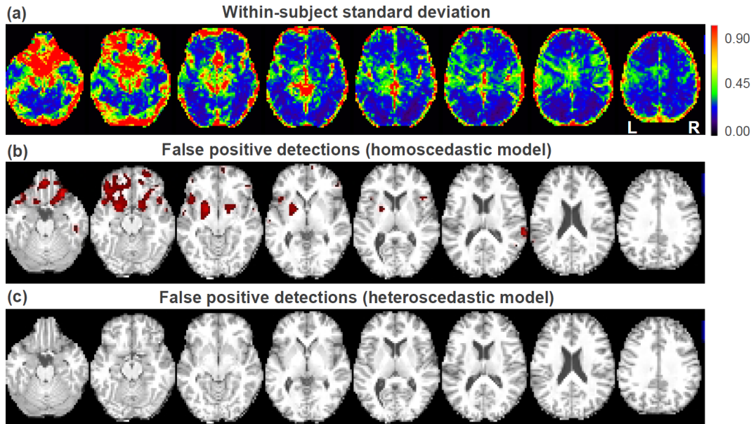
Figure 4: a) Estimated within-subject standard deviation in a control subject presenting locally atypical values. b) T1w map with false positive detections (in red) by leave-one-out cross-validation (smoothing FWHM = 8 mm 3 ) with the homoscedastic model (b) and the heteroscedastic model (c). No false positive detections are observed with the heteroscedastic model.
