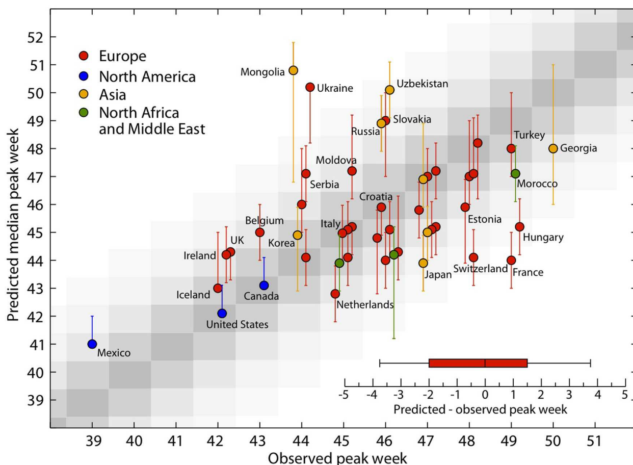
Figure 6 Statistical association between the predicted and observed activity peaks. Peak week as simulated by the model in the baseline stochastic forecast output (SFO) set with \alpha_{\min} = 0.65 versus the peak week observed by surveillance systems in the countries outlined in Figure 5. The reference ranges of the simulated peak week were obtained by analysis of 2,000 stochastic realizations of the model. In the inset, we show the box plot indicating the distribution of the differences between the simulated peak week for the baseline SFO set with \alpha_{\min} = 0.65 , and the observed peak week.
