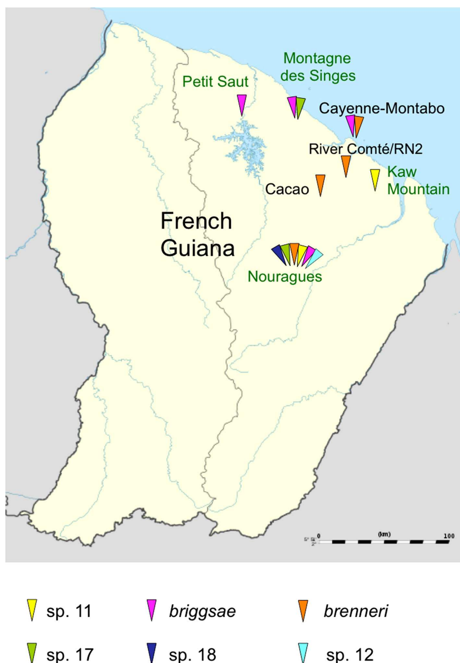
Figure 1 Sampling of Caenorhabditis species in French Guiana. The triangles indicate the presence of different Caenorhabditis species in the sampled areas, colour-coded as indicated in the legend. The names of locations with strong human activity (e.g. towns and villages) are written in black, and other locations (e.g. forests) in green.
