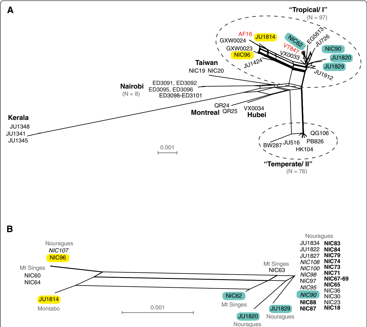
Figure 5 Neighbour-network based on the concatenated sequences of six nuclear loci depicting the relationships among C. briggsae isolates isolated worldwide (A) and from French Guiana (B). (A) Pattern of global C. briggsae diversity from a worldwide collection of 189 isolates (57 new from this study). Selections of isolates are labelled for reference; reference isolates AF16 and VT847 are indicated in red. Reticulation indicates potential recombination among isolates. (B) French Guiana isolates are partitioned into two groups that do not reflect the spatial distribution between the sampling sites but that correspond to the more general clustering observed within the “Tropical/I.” A subset of isolates is colour-coded similarly (yellow or blue) on both panels for reference. Isolates in bold derive from the subsampling of Cecropia H3, those in italics of H6. Note that only isolates with sequence information across the set of six loci were used to infer relationships among isolates.
