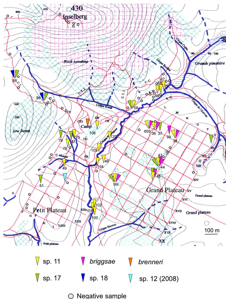
Figure 3 Spatial distribution of Caenorhabditis species in the Nouragues Natural Reserve. Triangles indicate the presence of a Caenorhabditis species, colour-coded as indicated in the legend. Numbers next to the triangles correspond to the GPS coordinate identifier (see Additional file 2). Small grey dots indicate spots containing only negative samples, i.e. samples lacking Caenorhabditis .
