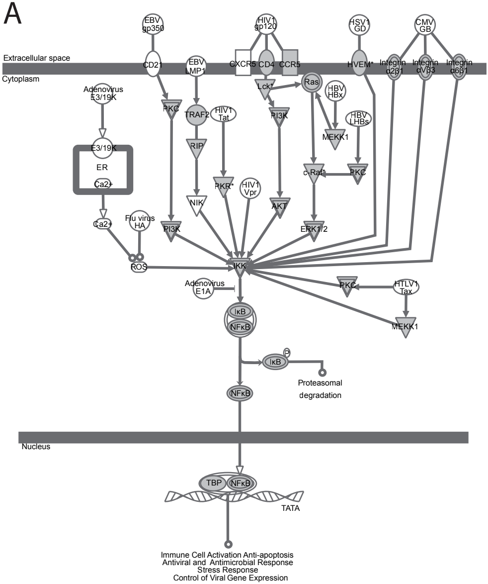
NF-κB activation by viruses pathway: -\log(q\text{-value}) = 6.26
