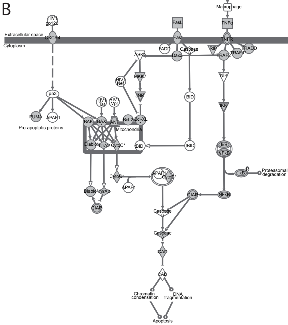
Induction of apoptosis by HIV1 pathway: -\log(q\text{-value}) = 5.64
