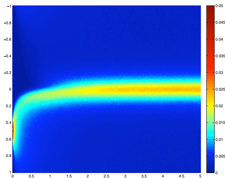
Figure 2 Transient distribution. Simulation of \rho(t,x) for t \in [0:5] and x \in [-1:1] . Setting \rho(0,x)=\delta(x-0.5) as the initial condition. The diffusion profile is as in Figure 1 and therefore the distribution obtained near t=5 is the same as the one at equilibrium described in Figure 1.
